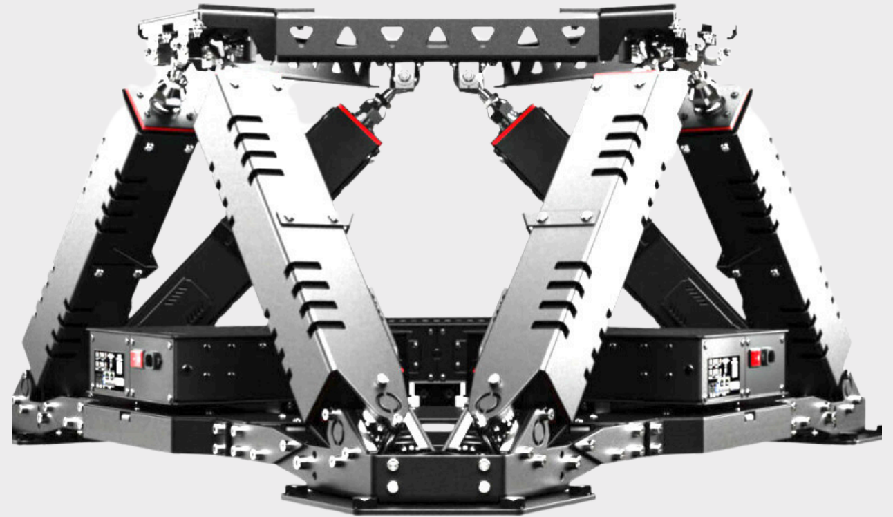
6 Degrees of Freedom (DOF) 1.5-4.5" motion by Qubic
